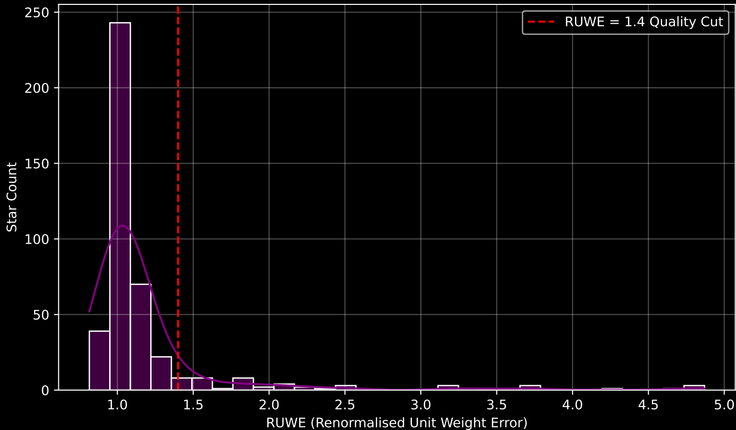
GALAH DR4 Field [9394] RUWE Distribution (n= 423)
