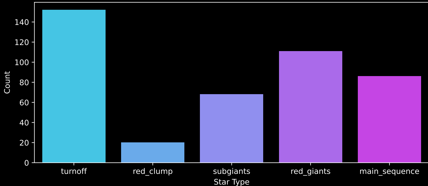
GALAH DR4 Field: [9394] Count plot of Star Type
