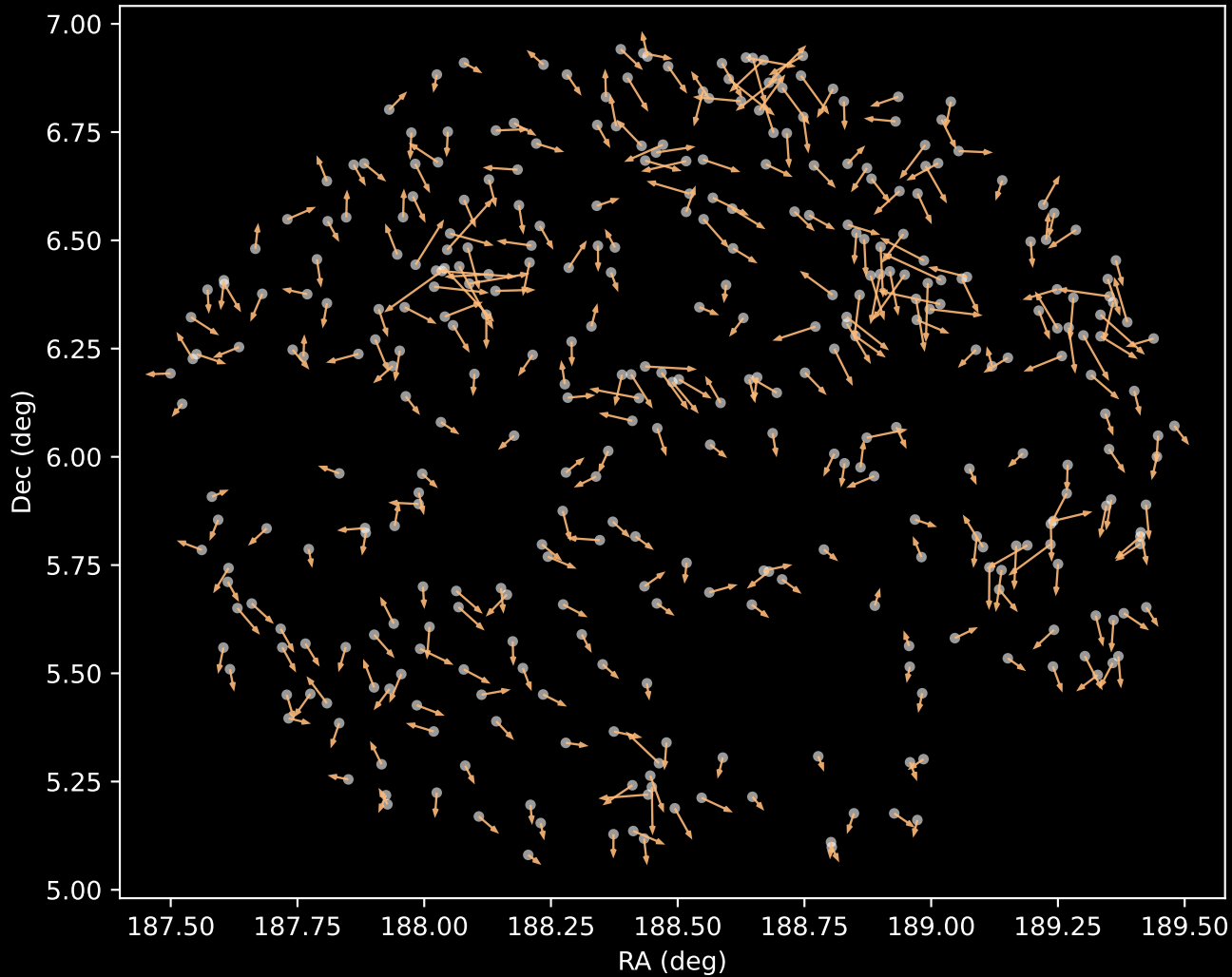
GALAH DR4 Cluster 3 Proper Motion Vectors (n=357)
